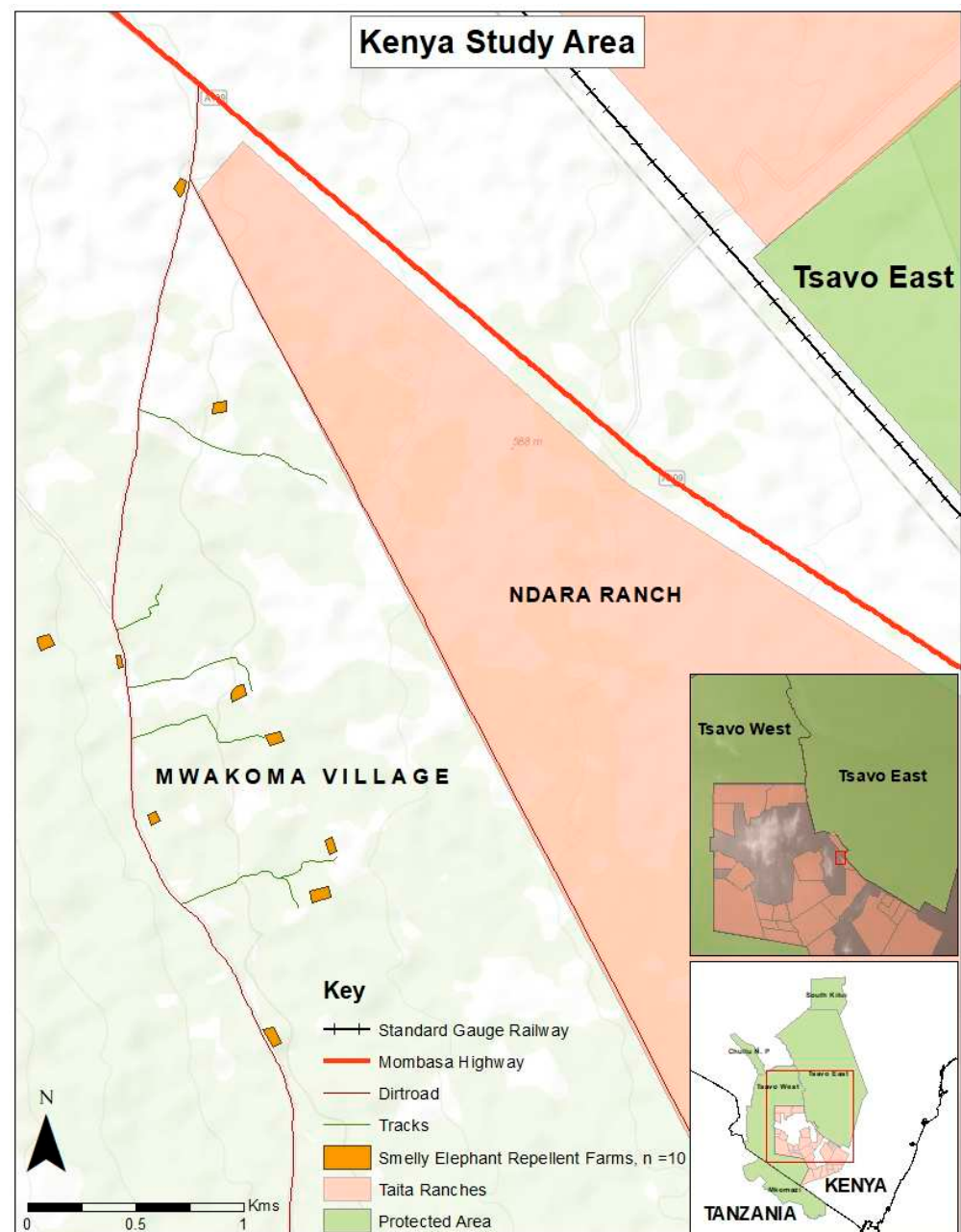
Figure 2. Location of the 10 smelly elephant repellent test farms in Mwakoma Village, Lower Sagalla, Taita-Taveta County, Kenya.
